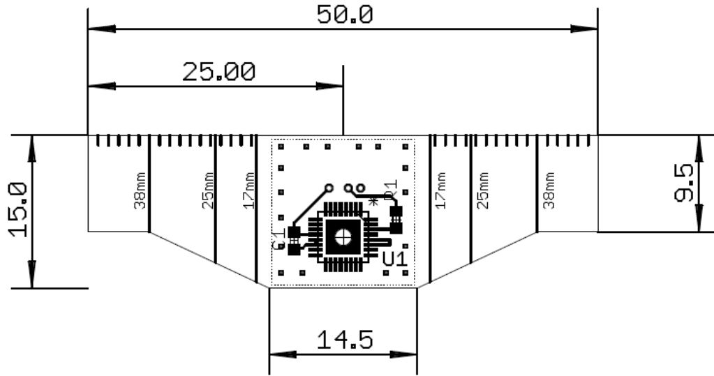
Figure 10: Example of an MFB-Sensor PCB
