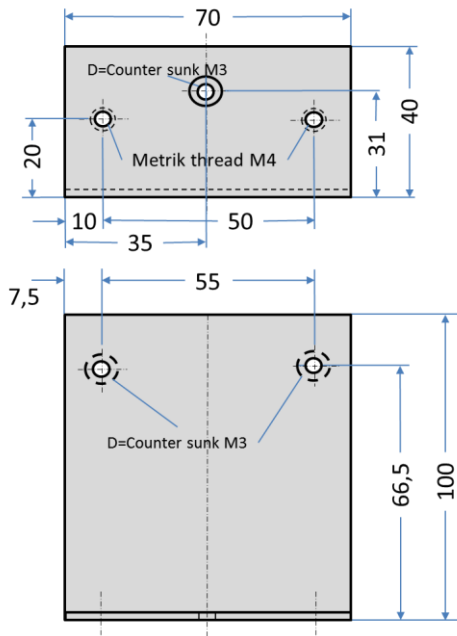
Figure 8: Mounting Flange (Ver. 1)
