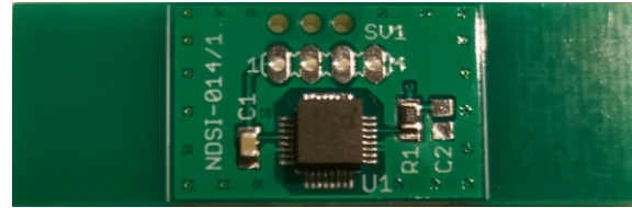
Figure 5: MFB-Sensor PCB
